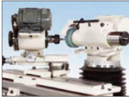
Radius grinding attachment
