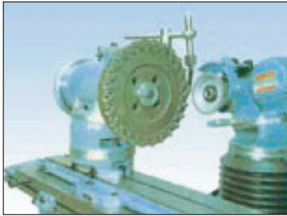
Face mill grinding attachment
