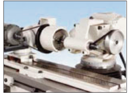
Internal grinding attachment
