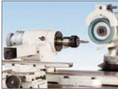
Helical grinding attachment
